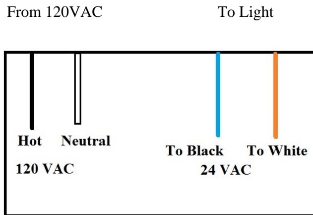
LED Transformer Box Connections
